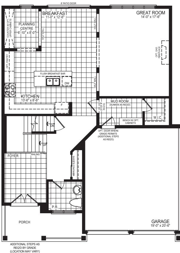
GROUND FLOOR PLAN STYLE A
