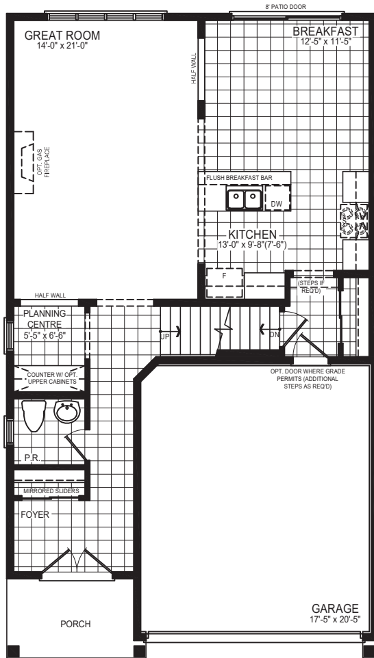
GROUND FLOOR PLAN STYLE A
