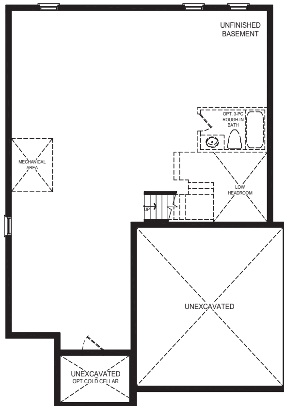
BASEMENT PLAN STYLE A
