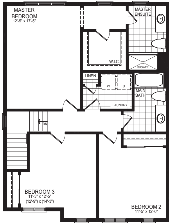
SECOND FLOOR PLAN STYLE A
