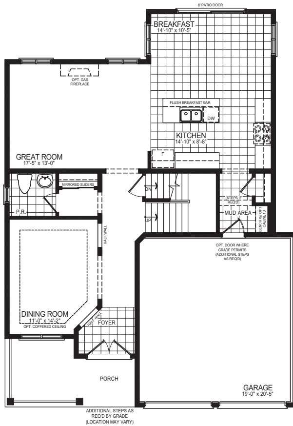
GROUND FLOOR PLAN STYLE A
