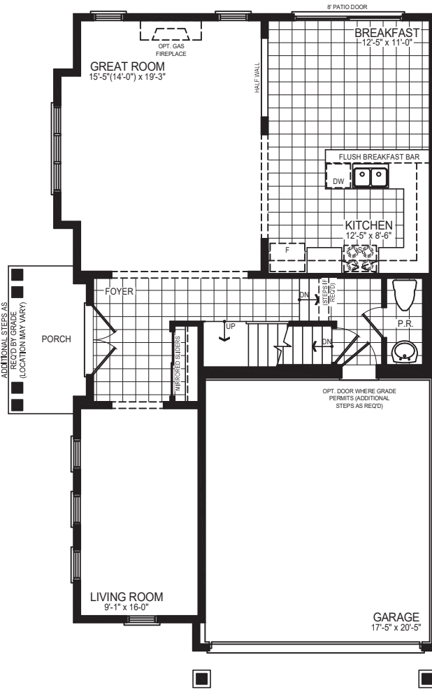
GROUND FLOOR PLAN STYLE A
