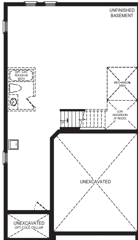
BASEMENT PLAN STYLE A
