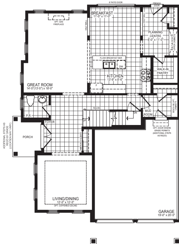
GROUND FLOOR PLAN STYLE A
